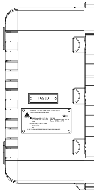
Left View
