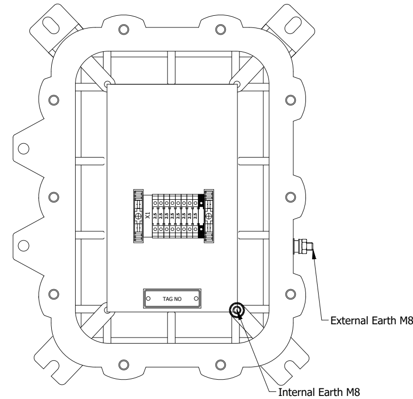
Internal View
