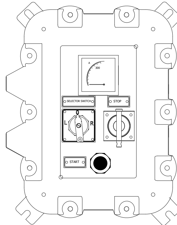
External View
